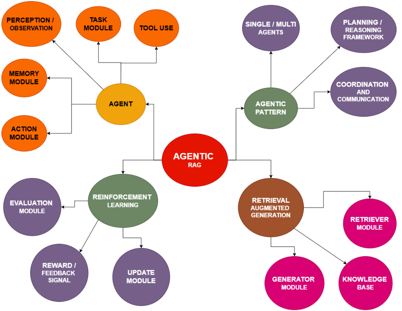
Fig. 3: Agentic-RAG + Reinforcement Learning
